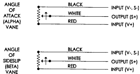
ELECTRICAL SCHEMATIC
